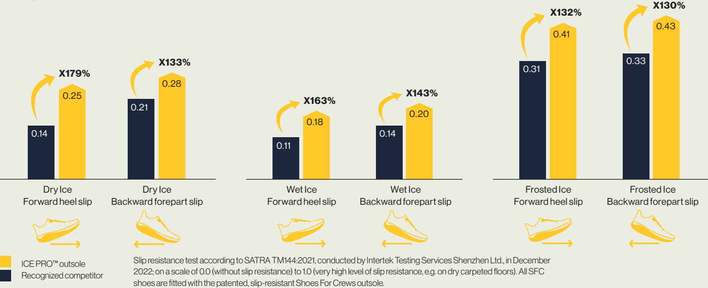
Testing the slip resistance of our ICE PRO™ OUTSOLE on ice [SATRA TM144:2021]
