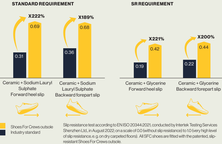
Testing the slip resistance of our SFC OUTSOLE [EN ISO 20344:2021]
